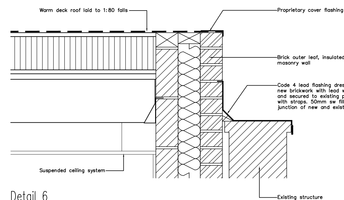
Detail 6 Scale 1:10 @ A1
